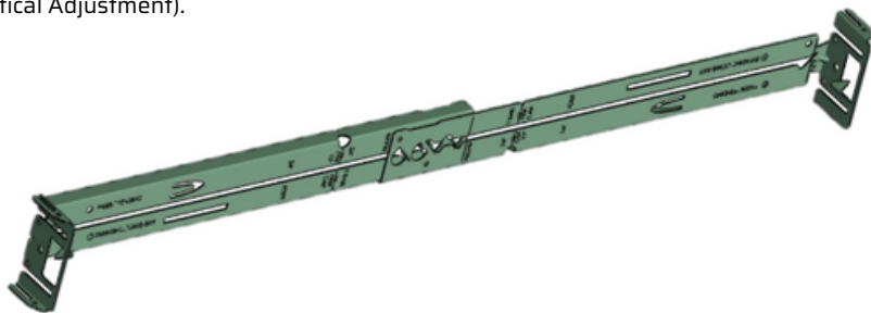
Fig. 72 Set of two L-Bars #1487, 4 required per Plaster Frame Assembly
