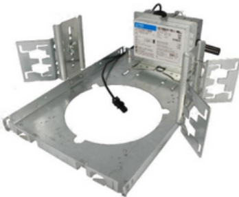
Fig. 35 Plaster Frame with junction box
