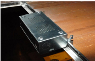
Fig.79 Mounted to Plaster frame with Driver installed to cover
