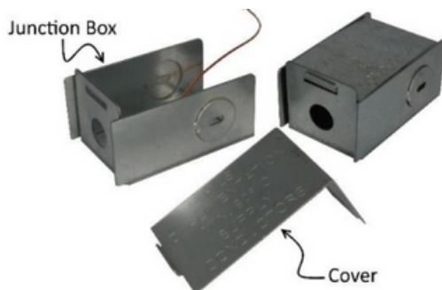
Fig. 50 1257-1 Junction Box & 1258 Cover
