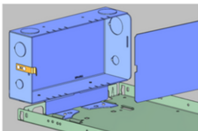
Fig. 45 1432 Junction Box
