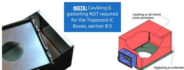
Fig. 56 1681-XX or 1685-XAT series Ultra-airtight IC Box (with integral gasketed junction box) with 1286-XAT series plaster frame mounted
