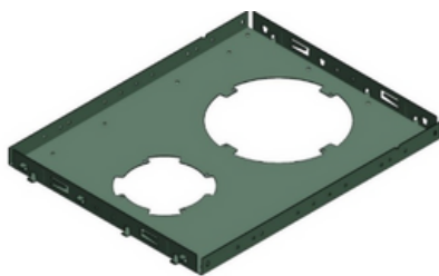
Fig. 25 1483-1-XX series Plaster Frame with double and irregular holes
