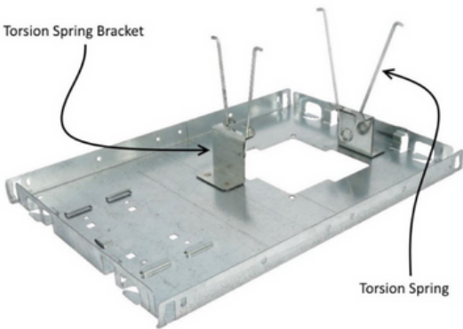
Fig. 16 Torsion spring brackets
