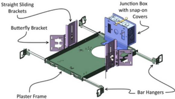
Fig. 18 Plaster frame assembly
