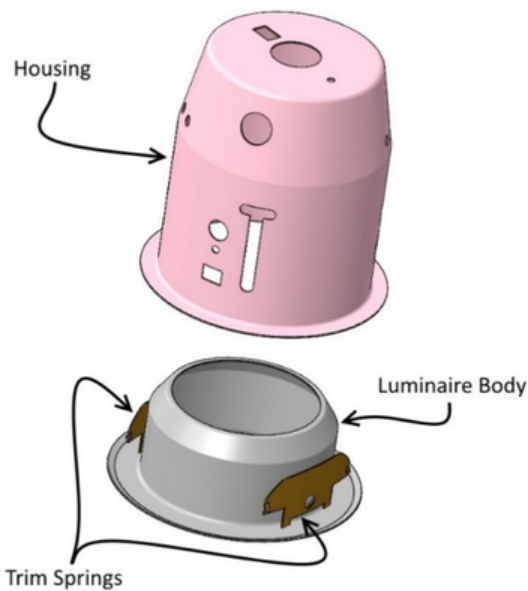
Fig. 14 Luminaire retention with curved trim springs
