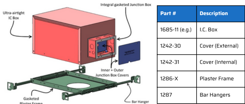
Fig. 6 Typical Ultra-airtight IC Box with integral gasketed junction box & gasketed plaster frame
