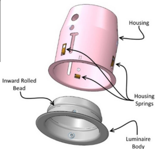
Fig. 13 Luminaire retention with housing springs
