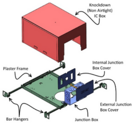
Fig. 4 Non-airtight IC Box placed behind plaster frame assembly containing integral junction box & junction box covers
