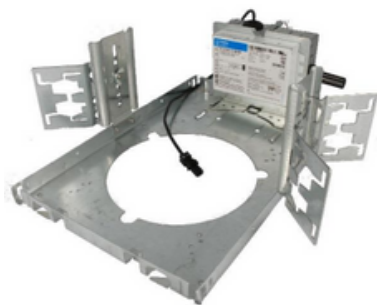
Fig. 73 Plaster frame with Straight Brackets #1253 or 1253-4* & Butterfly Brackets #1254
